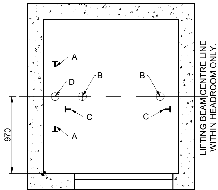
PIT PLAN [1:30]
