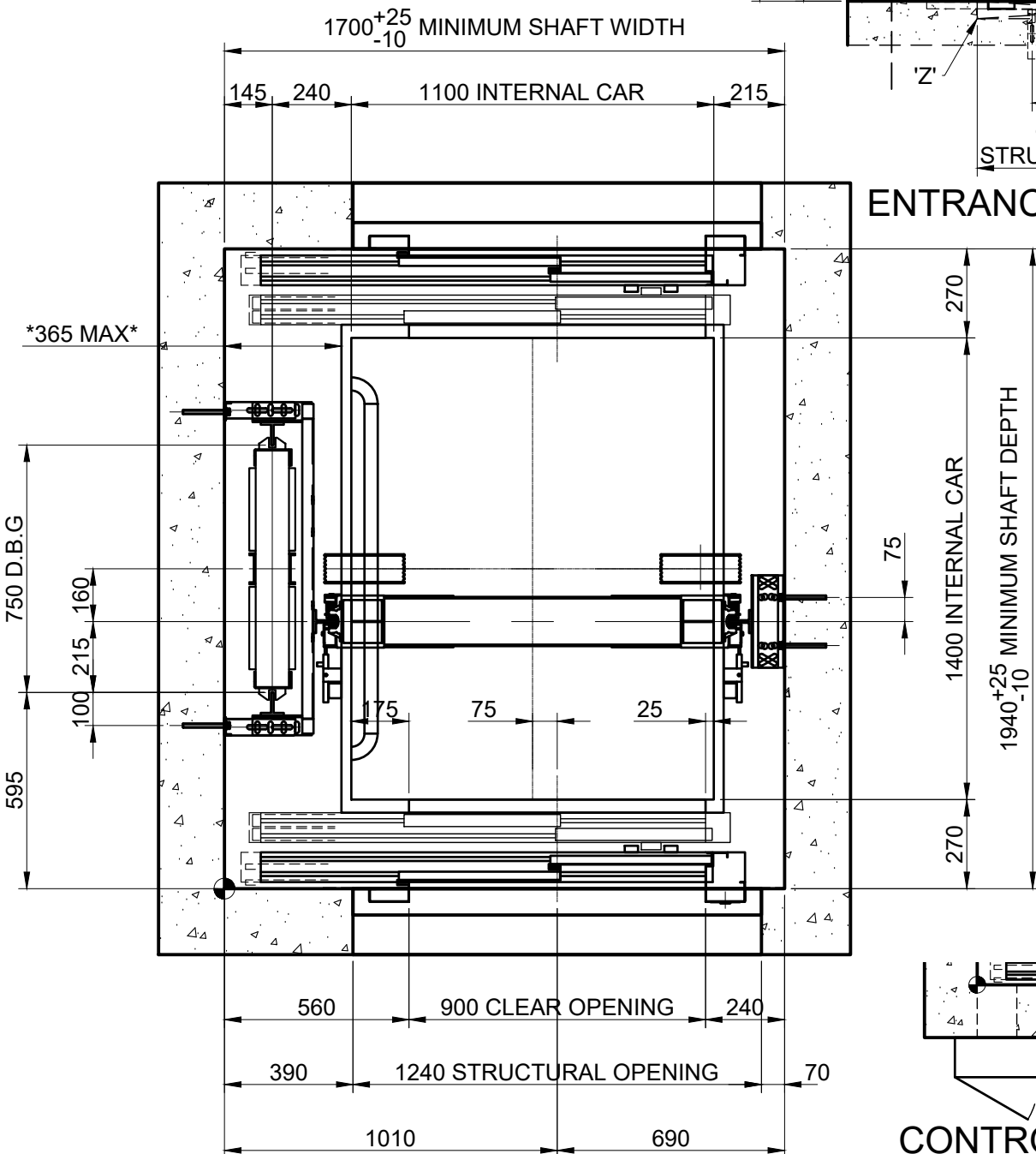
PLAN VIEW ON LIFT SHAFT [1:20]
