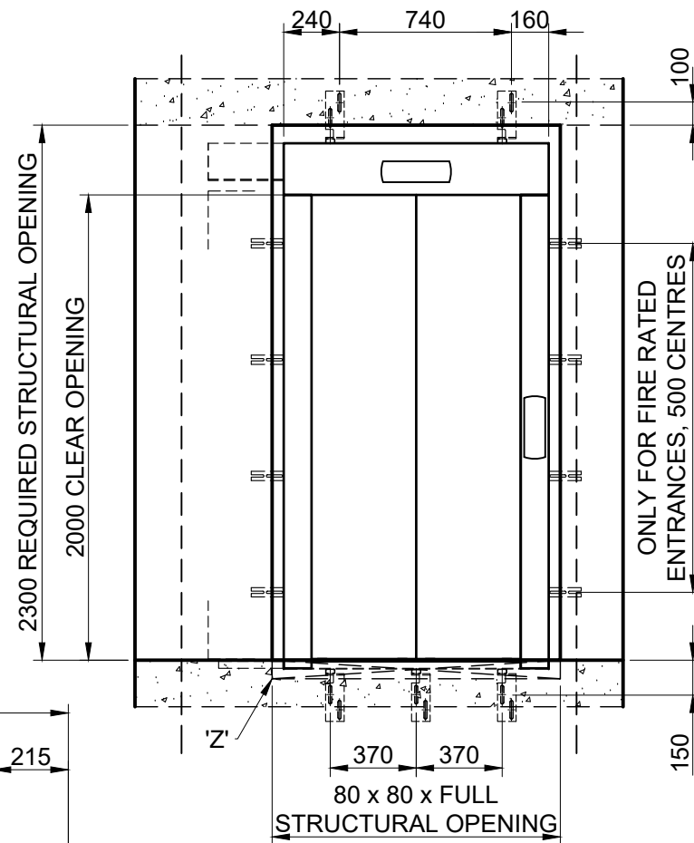
ENTRANCE DETAIL [1:30]
