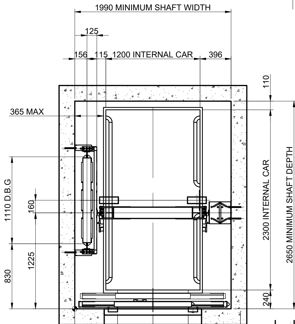
PIT PLAN [1:40]
