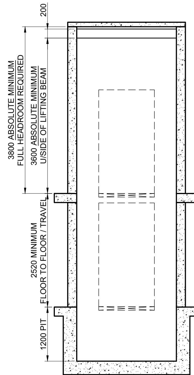
SECTIONAL ELEVATION A-A [1:50]
