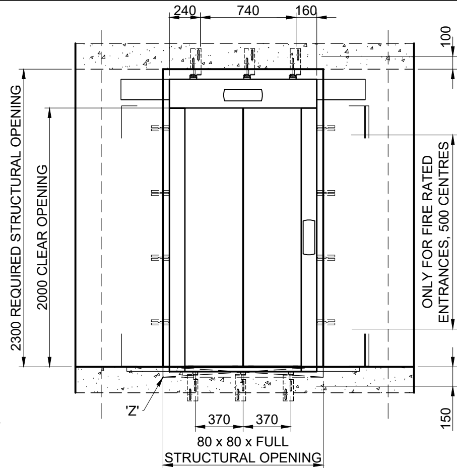
ENTRANCE DETAIL
