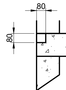
DETAIL Z [1:20]
