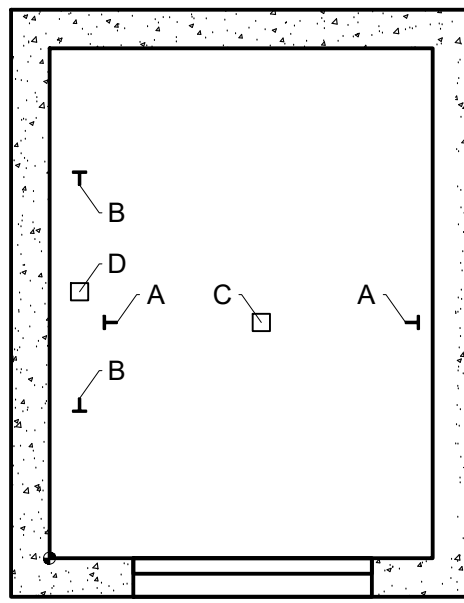
PIT PLAN [1:40]
