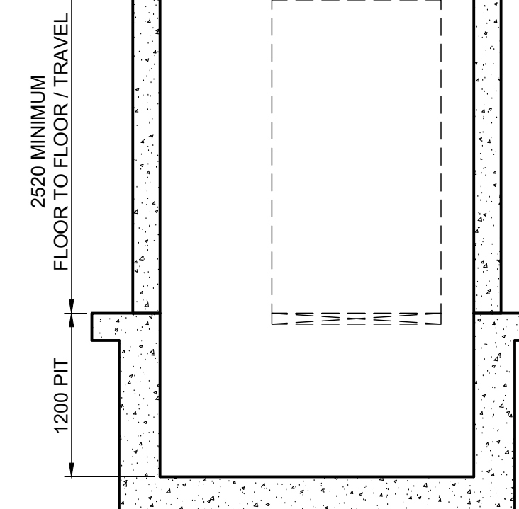
SECTIONAL ELEVATION A-A [1:40]
