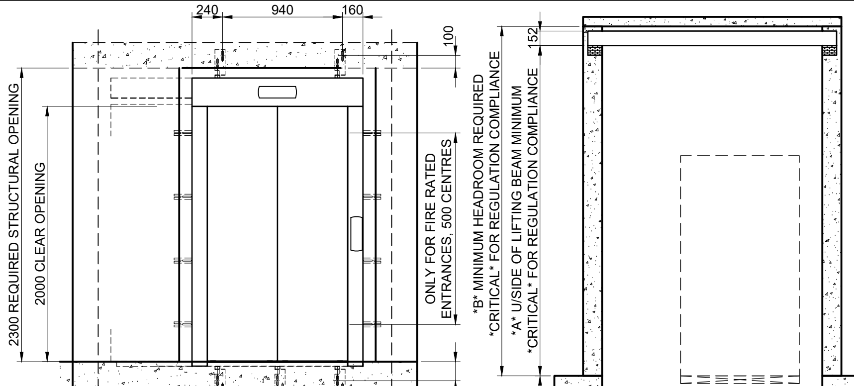
ENTRANCE DETAIL [1:30]
