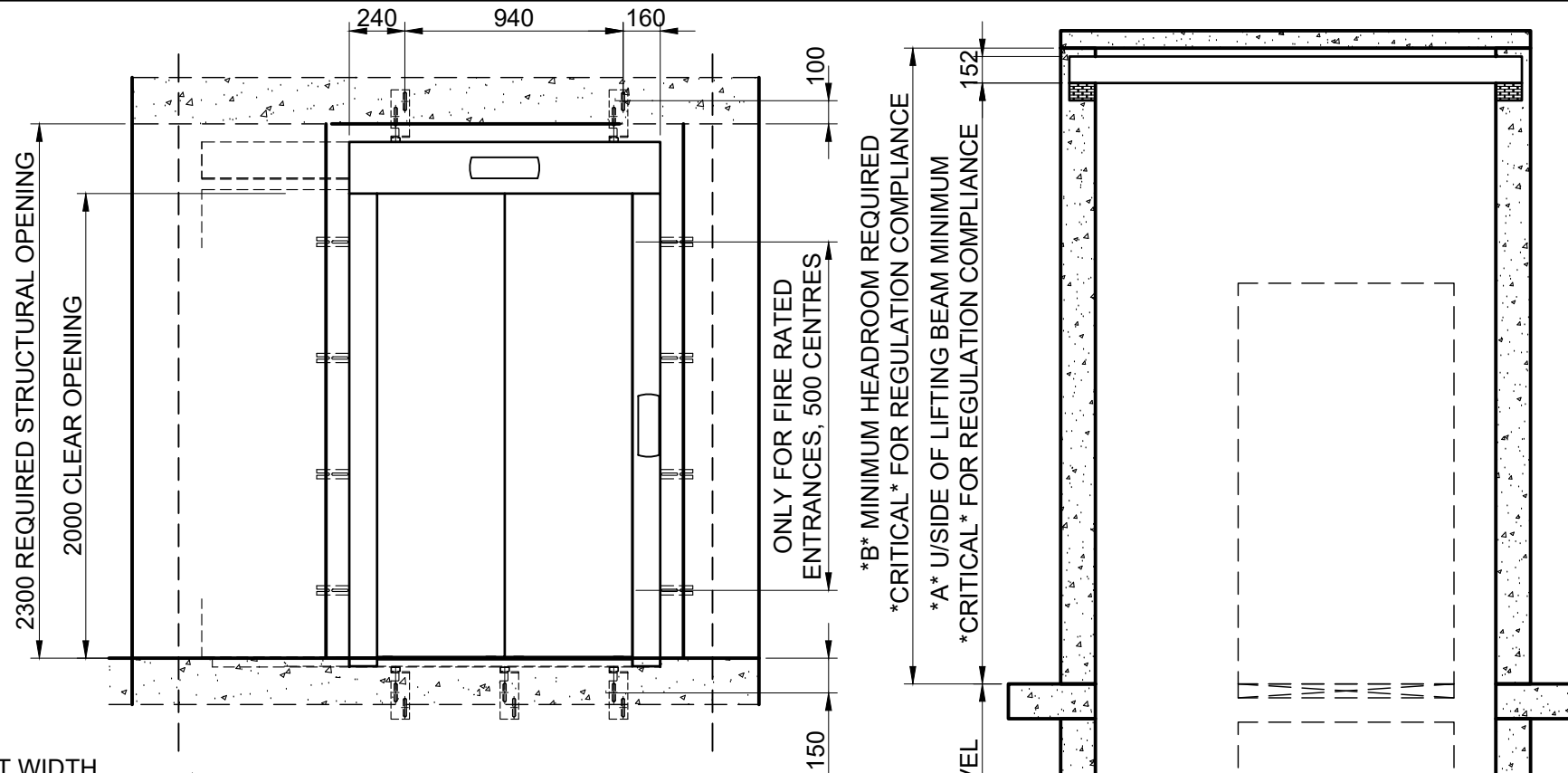
ENTRANCE DETAIL [1:30]
