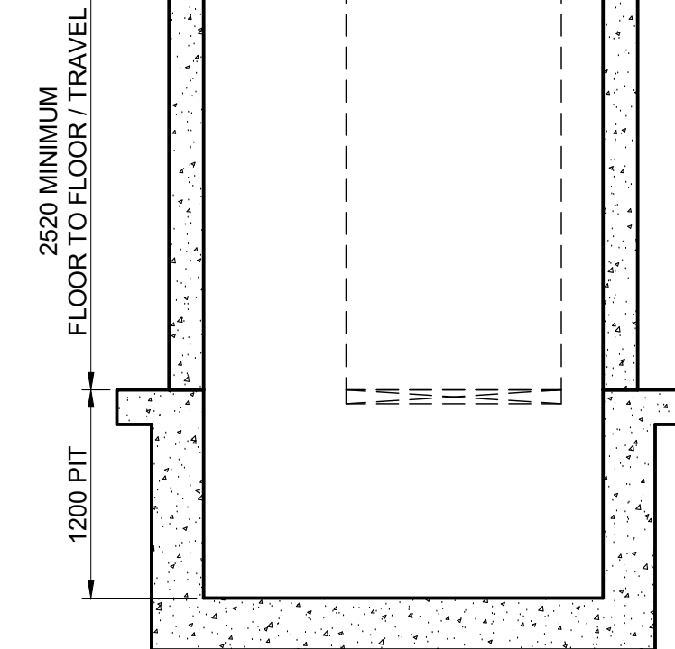
SECTIONAL ELEVATION A-A [1:40]
