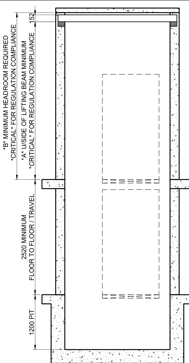
SECTIONAL ELEVATION A-A [1:40]
