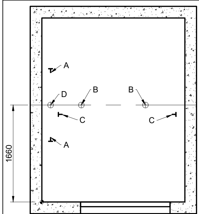
PIT PLAN [1:40]
