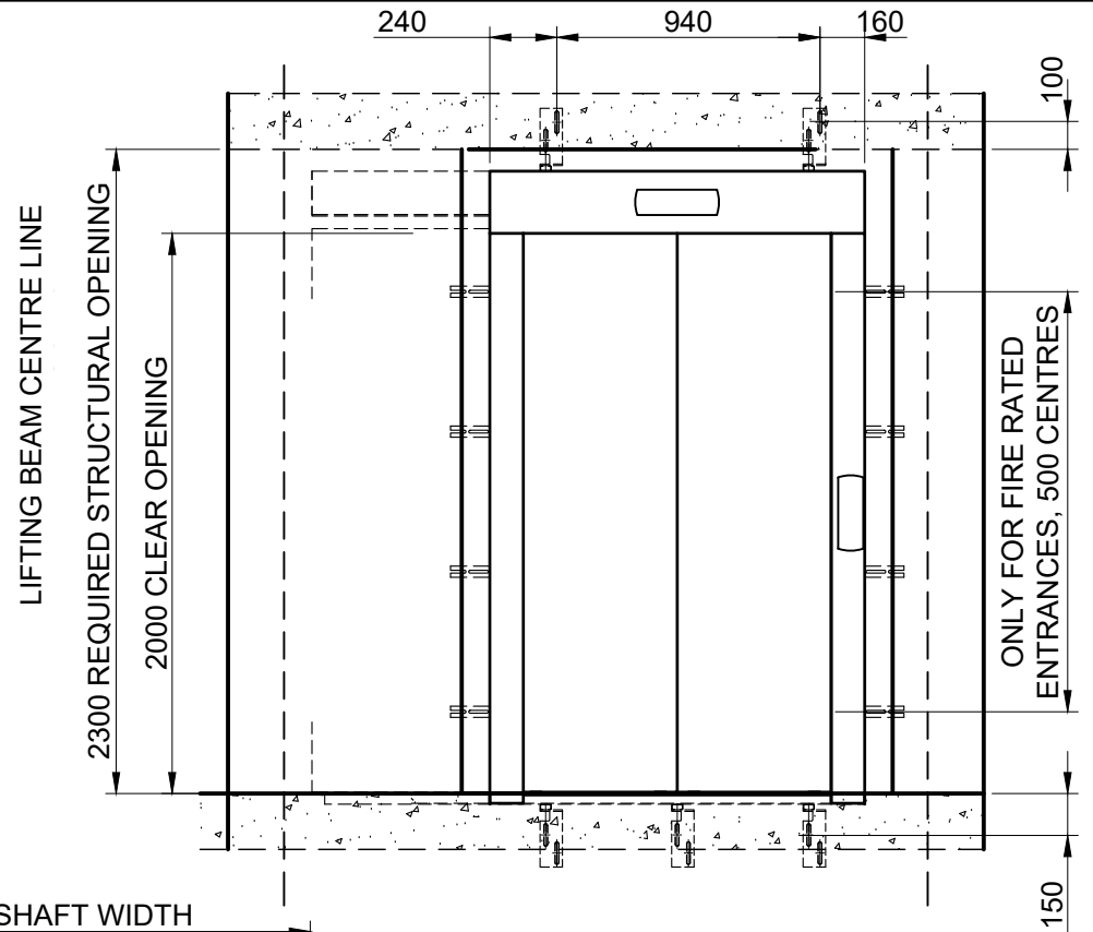
ENTRANCE DETAIL [1:30]
