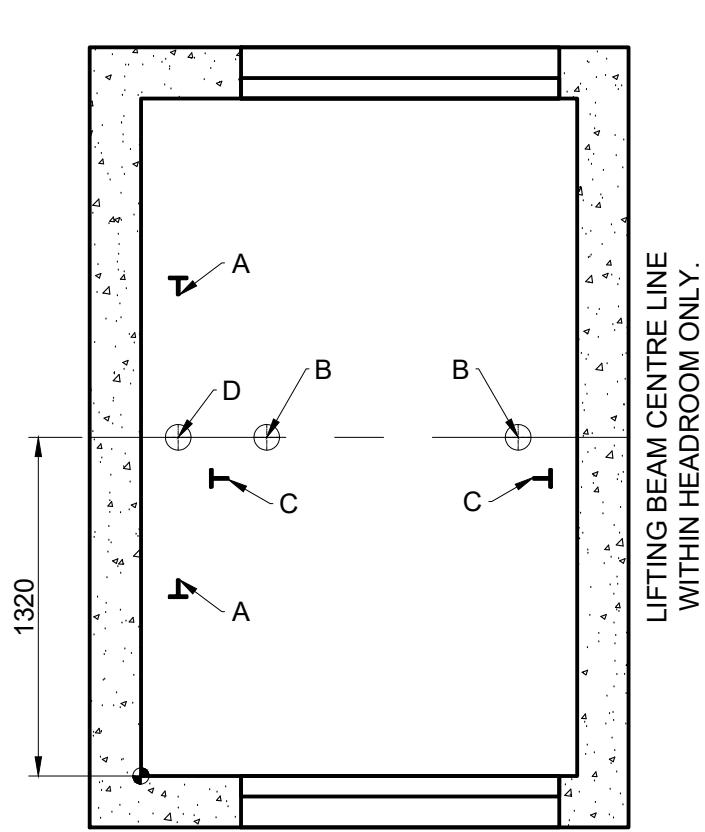
PIT PLAN [1:30]
