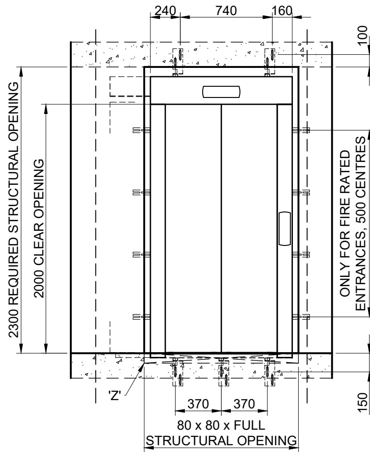
ENTRANCE DETAIL [1:30]
