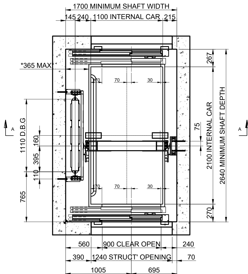
PLAN VIEW ON LIFT SHAFT [1:30]
